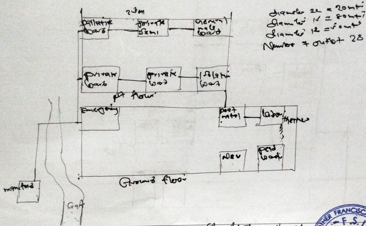
PROPOSED PIPING ROUTE DRAWING FROM THE MANIFOLD TO THE POINT OF USE
