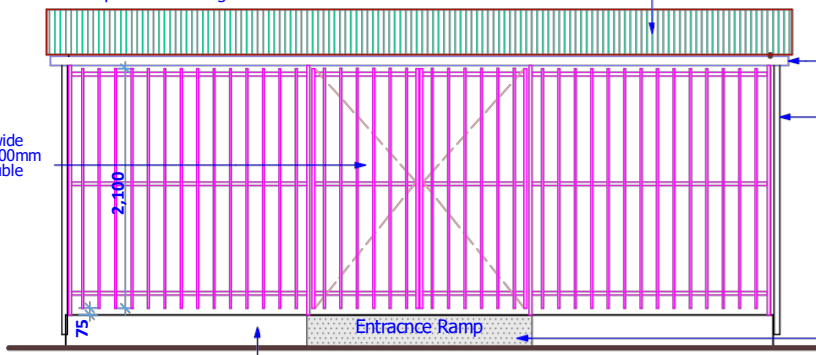
ENTRANCE ELEVATION 01
