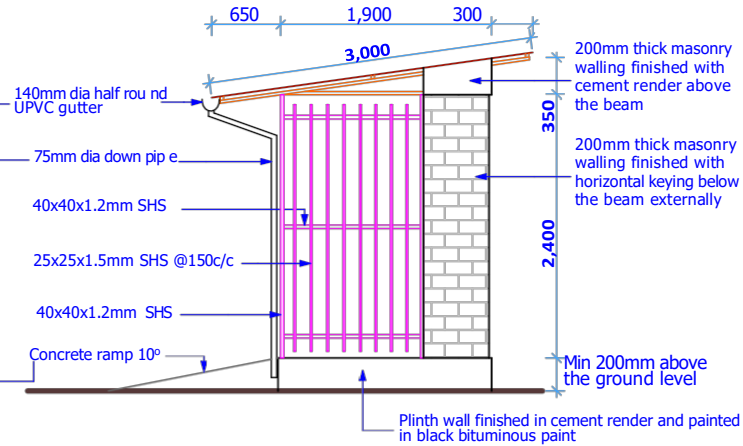
SIDE ELEVATION 02
