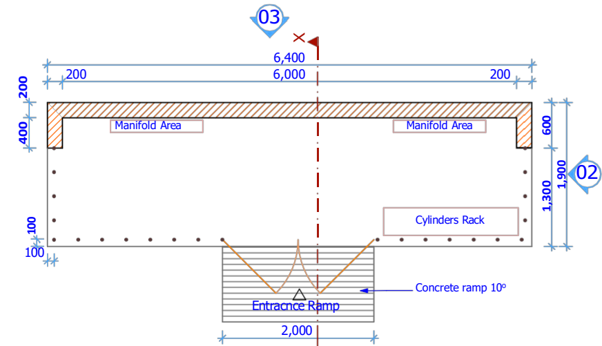
FLOOR PLAN 01
